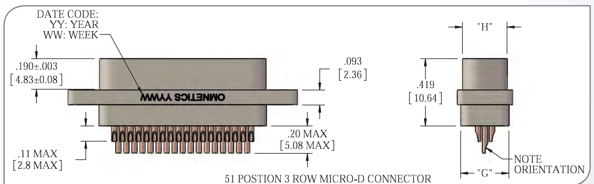
51 POSITION 3 ROW MICRO-D CONNECTOR
